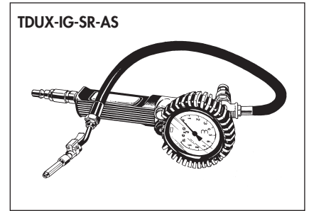
B Inflation gun to be connected to pressurized air bottle, pump or compressor. The inlet pressure to the inflation gun should be min. 4 bar/60 p.s.i. and max. 10 bar/150 p.s.i..
