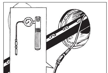
5.9 Inflate TDUX up to the pressure of 3,0 bar/45 p.s.i. and keep the pressure at 3,0 \pm 0,2 bar/ 45 \pm 3 p.s.i. during 30 sec. after which the tool must be shut-off.
