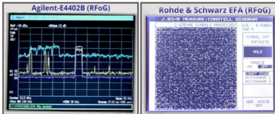
Figure 14: Measured Upstream RF Spectrum & constellation of probe channel with OBI in traditional RFoG
