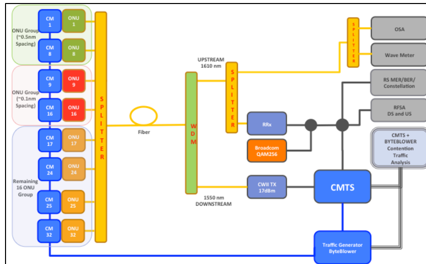
Figure 11: Comprehensive test bed to evaluate the effects of OBI
