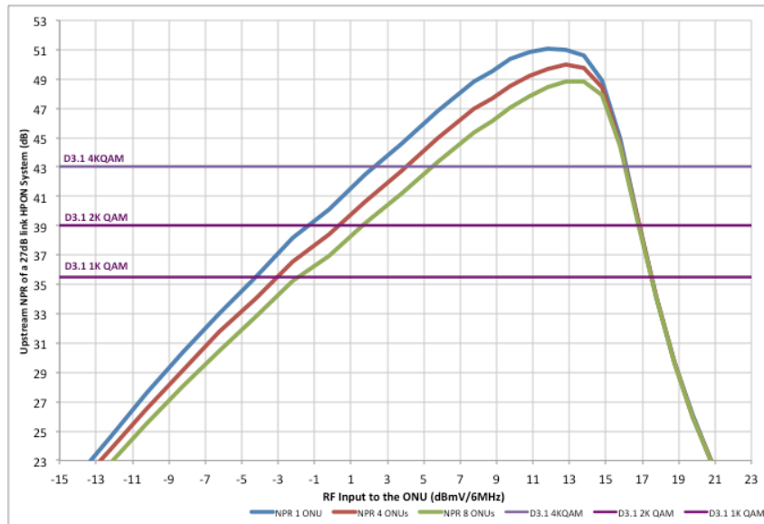
Figure 19: Measured NPR of a 25km, 27dB Link Budget 204 MHz HPON upstream system
