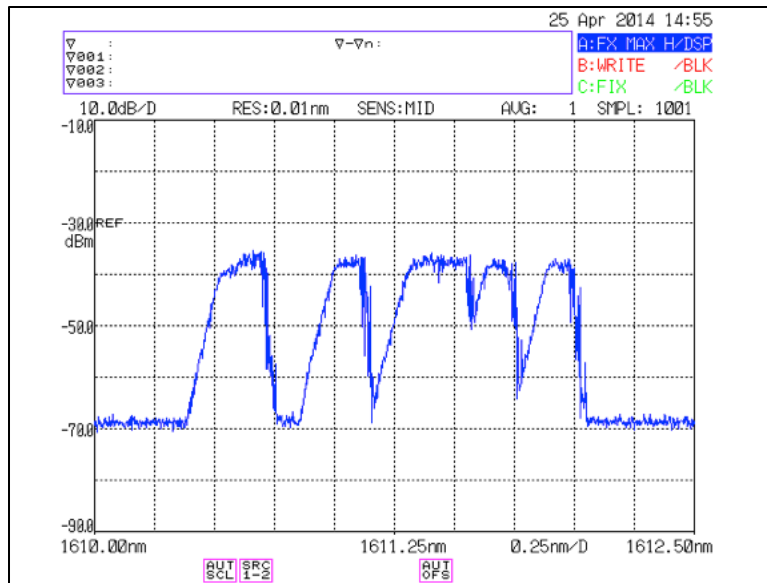
Figure 13: Measured optical spectrum under burst mode operation on Max Hold for traditional RFoG
