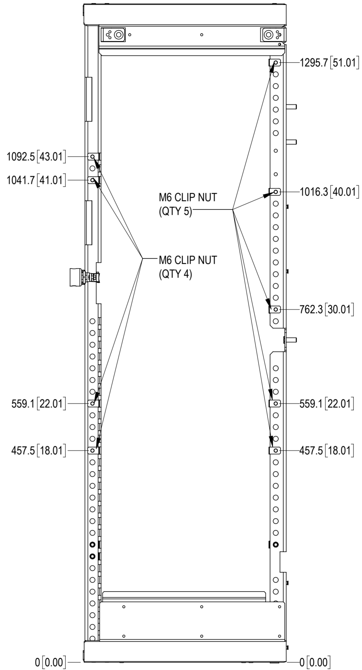
RIGHT SIDE VIEW (DOORS REMOVED)
