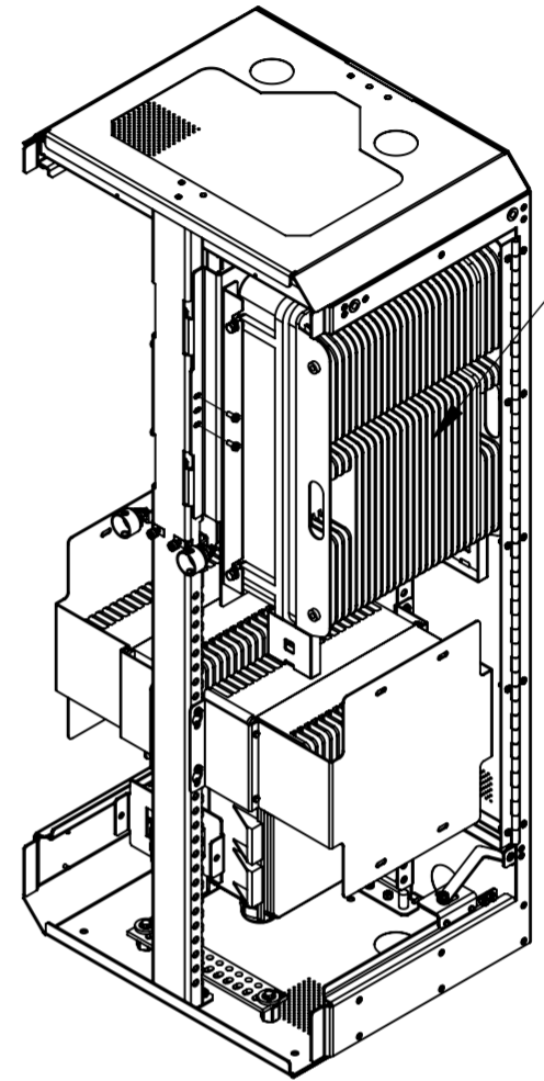
STEP 3: RIGHT AHLBBA HANG THIS ASSEMBLY TO THE EQUIPMENT MOUNT BRACKETS AND SECURE USING 5 SETS OF M6 HARDWARE, FLAT WASHER AND LOCK WASHER
