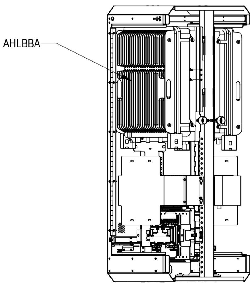
STEP 4: LEFT AHLBBA HANG THIS ASSEMBLY TO THE EQUIPMENT MOUNT BRACKETS AND SECURE USING 5 SETS OF M6 HARDWARE, FLAT WASHER AND LOCK WASHER
