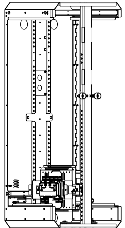
STEP 1: SDX1926Q-43 + RAYCAP HANG THIS ASSEMBLY TO THE EQUIPMENT MOUNT BRACKETS AND SECURE USING 3 SETS OF M6 HARDWARE, FLAT WASHER AND LOCK WASHER
