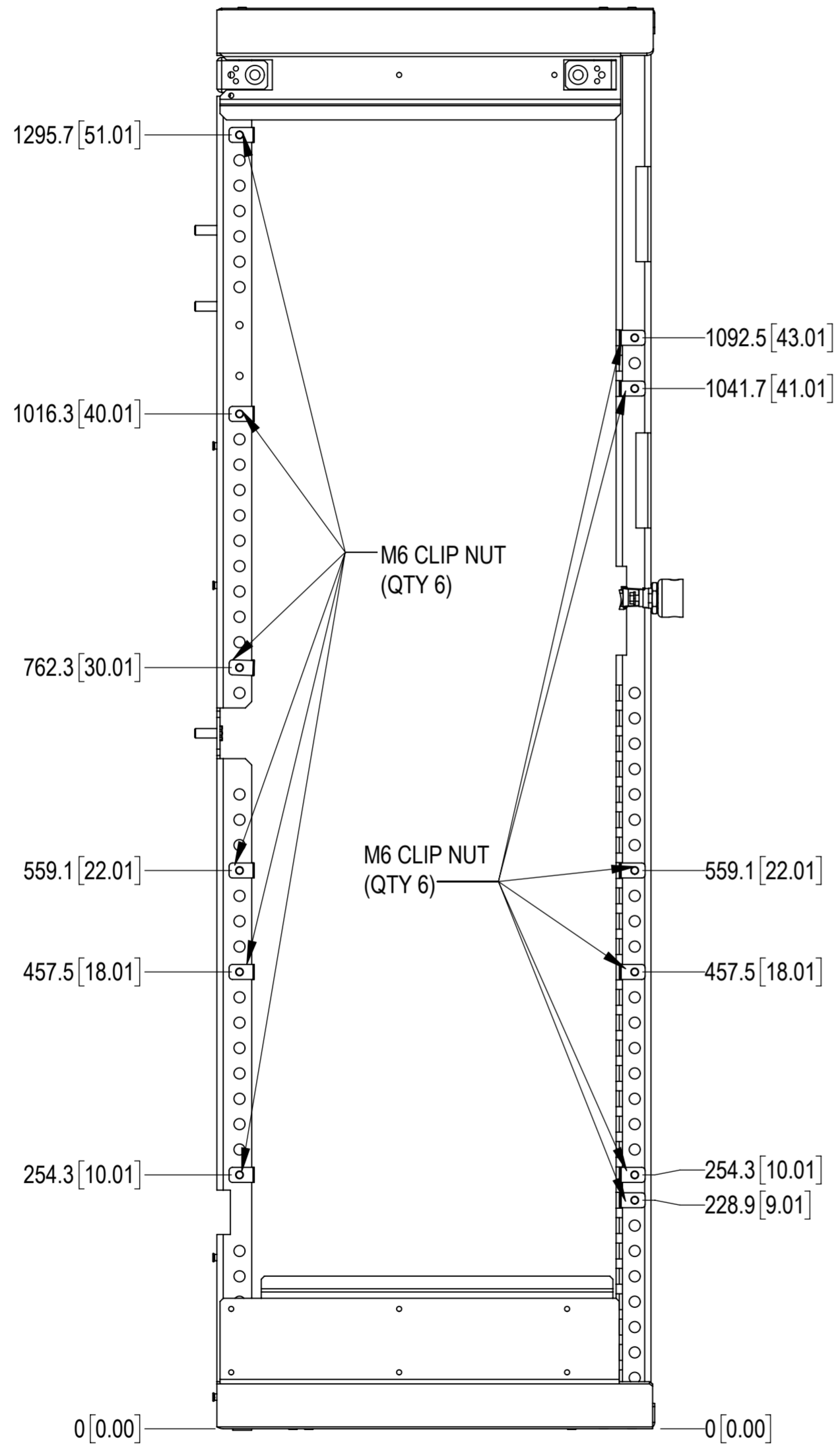
LEFT SIDE VIEW (DOORS REMOVED)
