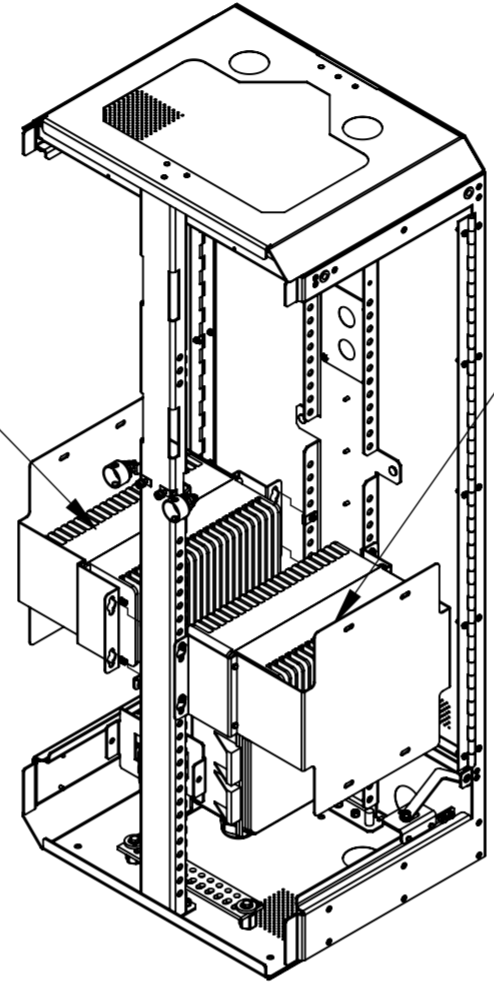
STEP 2: PSU-1200W-48-N HANG THIS ASSEMBLY TO THE EQUIPMENT MOUNT BRACKETS AND SECURE USING 4 SETS OF M6 HARDWARE, FLAT WASHER AND LOCK WASHER
