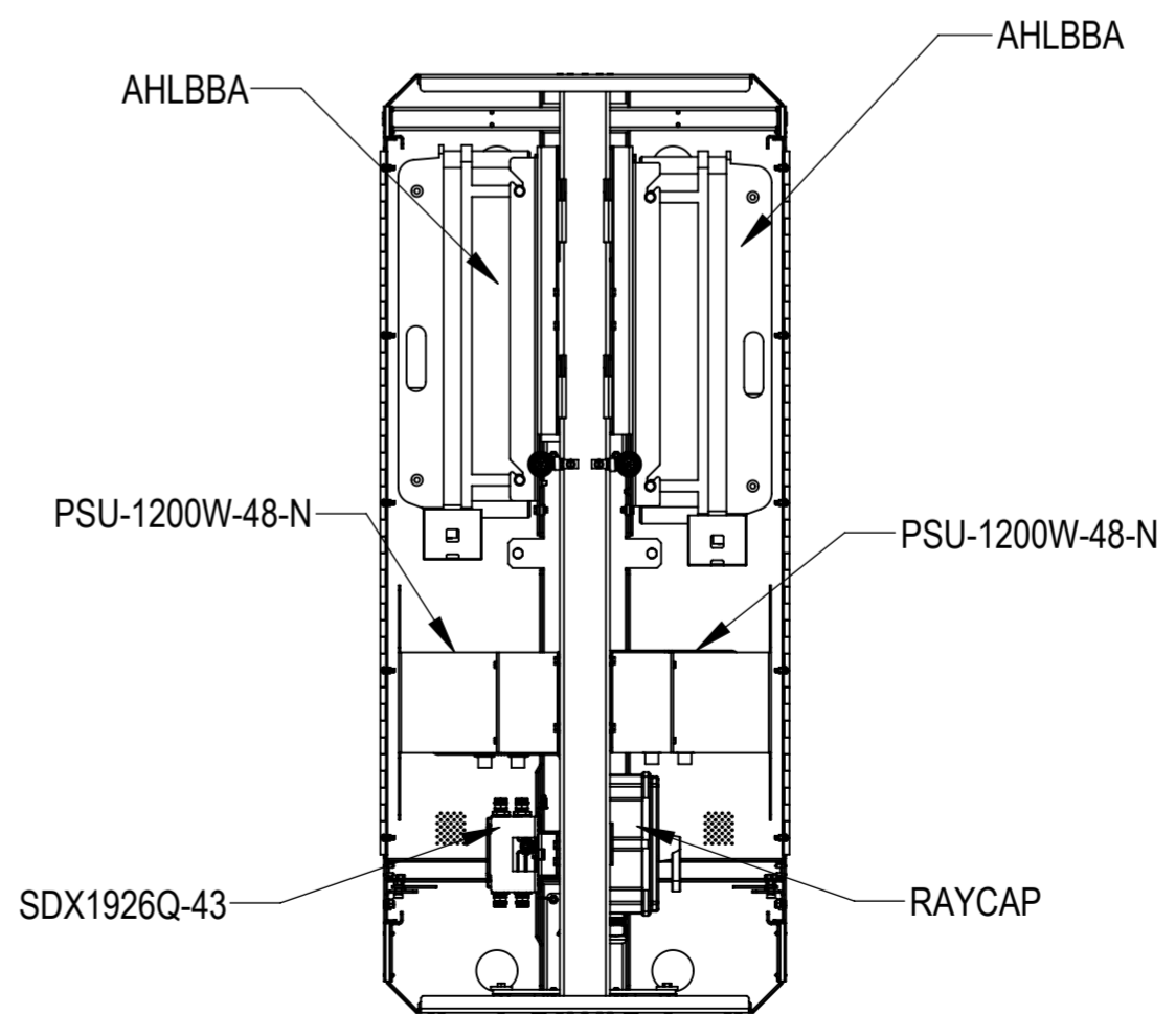
TOTAL INSTALLATION THE FRONT DOOR IS HIDDEN FOR CLEAR VIEWING
