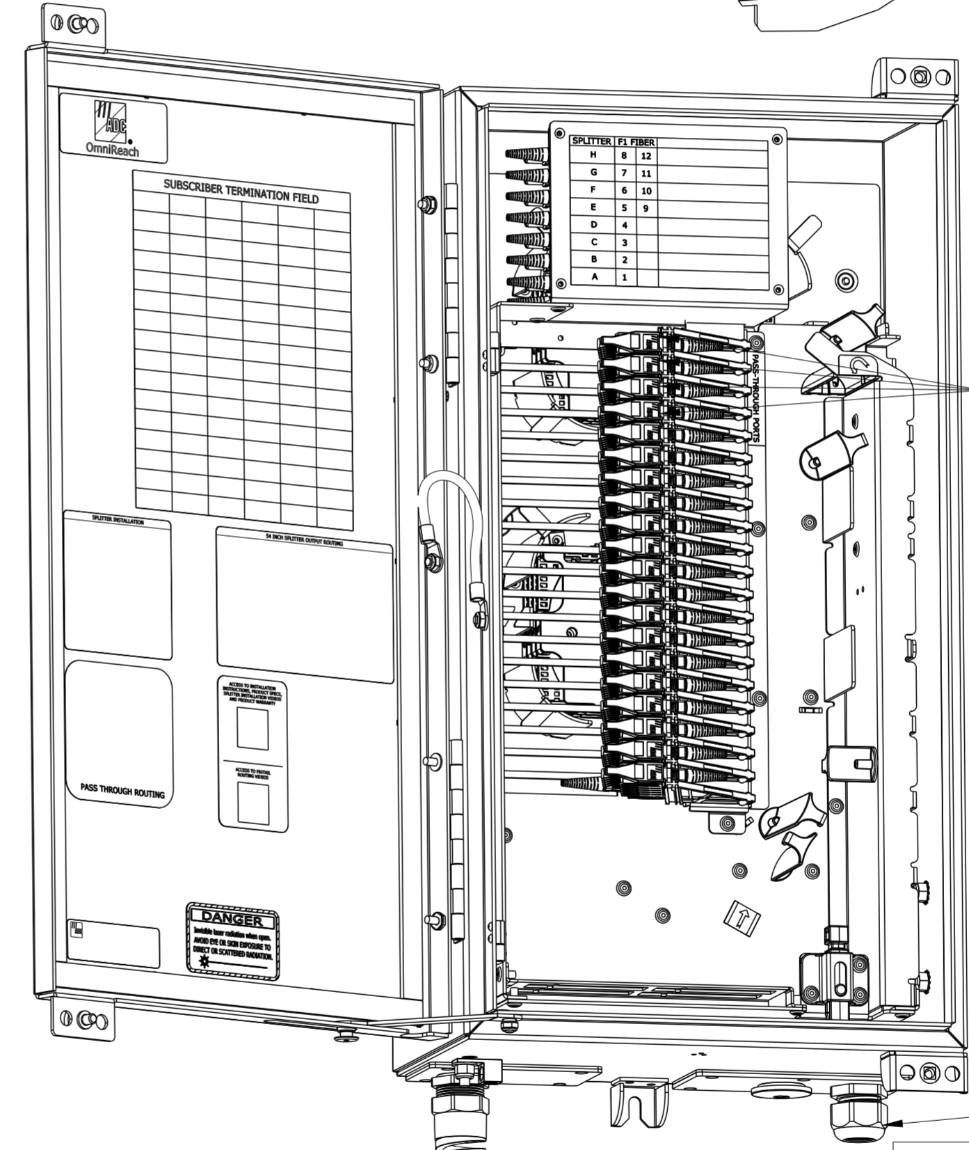
DISTRIBUTION STRAIN RELIEF FOR CABLES THAT ARE 0.35 TO 0.63 INCHES IN DIAMETER
