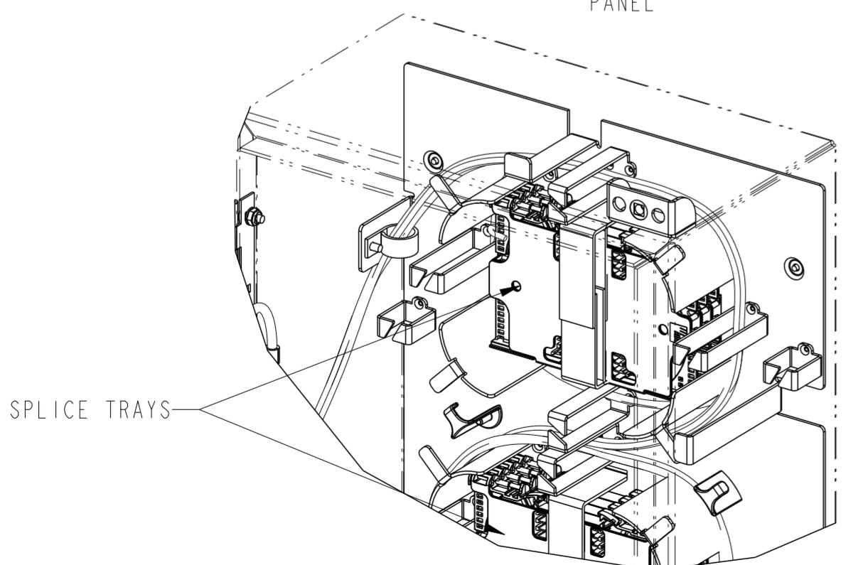
DETAIL A (SPLICE VERSION CABINET SHOWN WITH OPENED SWINGFRAME FOR REFERENCE ONLY)
