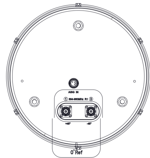
VIEW A-A BRACKET NOT SHOWN
