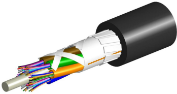
Fiber OSP cable, LightScope® ZWP Mini Single Jacket All-Dielectric, 96 fiber, Gel-Filled, Stranded Loose Tube, Singlemode G.652.D and G.657.A1, Feet jacket marking, Black jacket color
