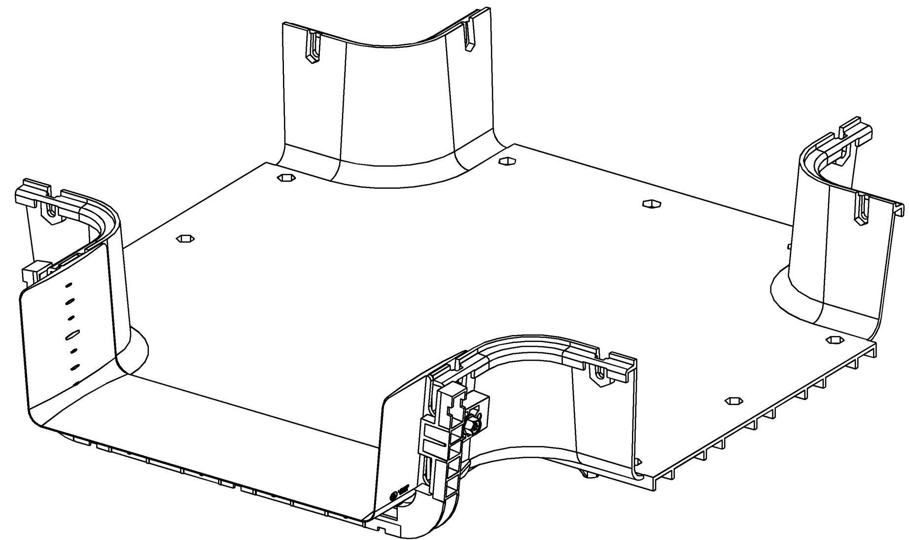
SCALE 0.375 COMPLETE ASSEMBLY
