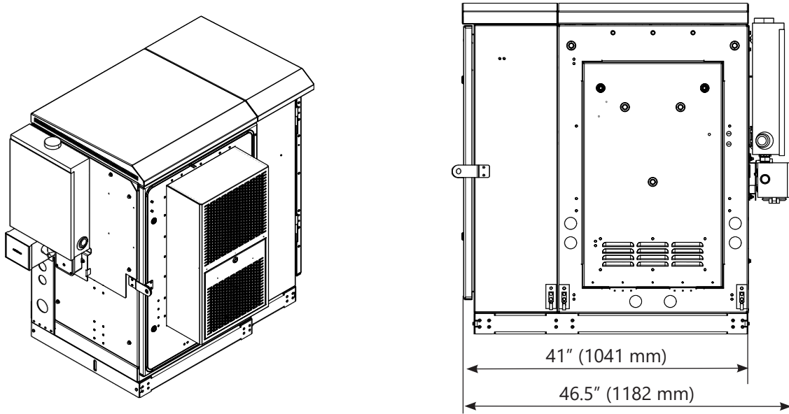
Figure 1. Isometric and Rear Views – CommScope Telco AIO Example
