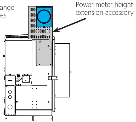
Figure 28. Structurally mounting power meters
