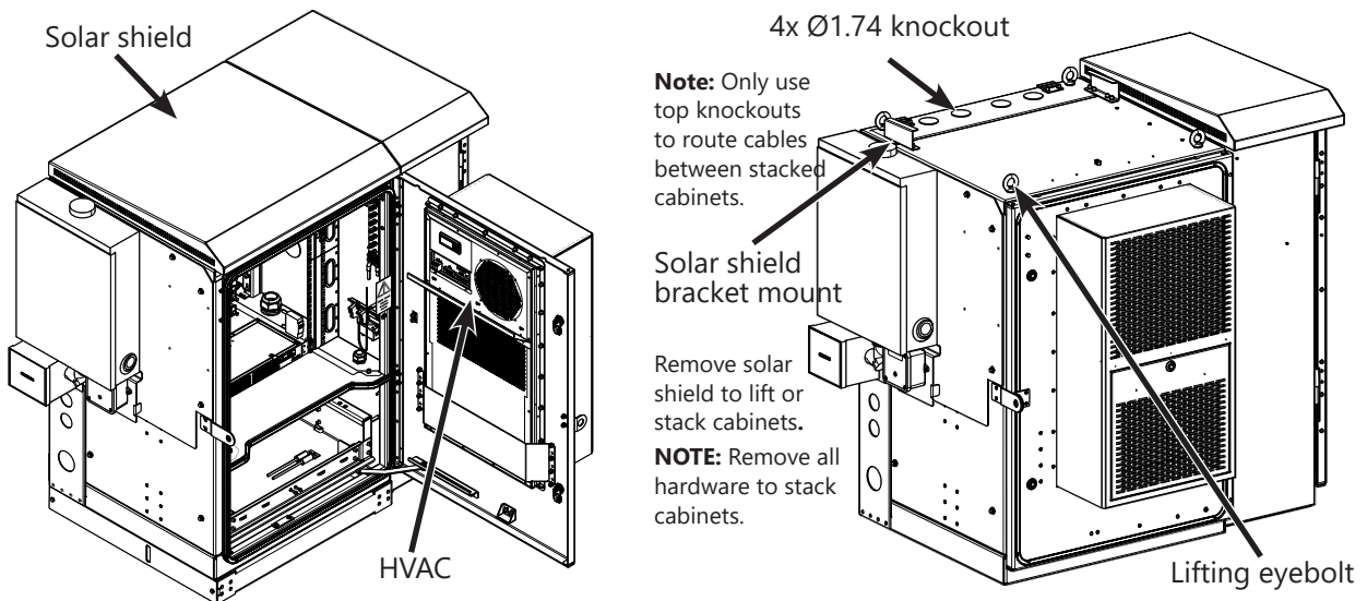
Figure 5. Equipment Cabinet with Solar Shield On or Off – CommScope Telco AIO Example
