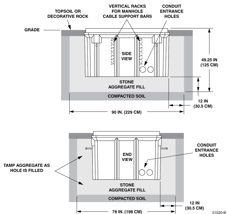
Figure 26. Excavation Recommendations for (FMS-FD3J-KIT-B)
