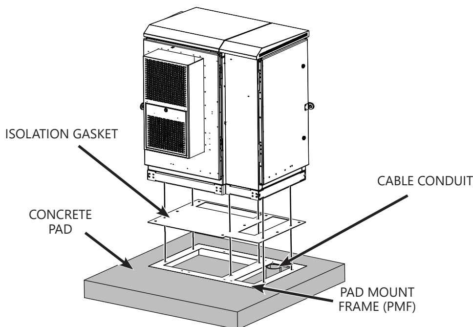
Figure 15. Mounting the All In One Cabinet on the Concrete Pad
