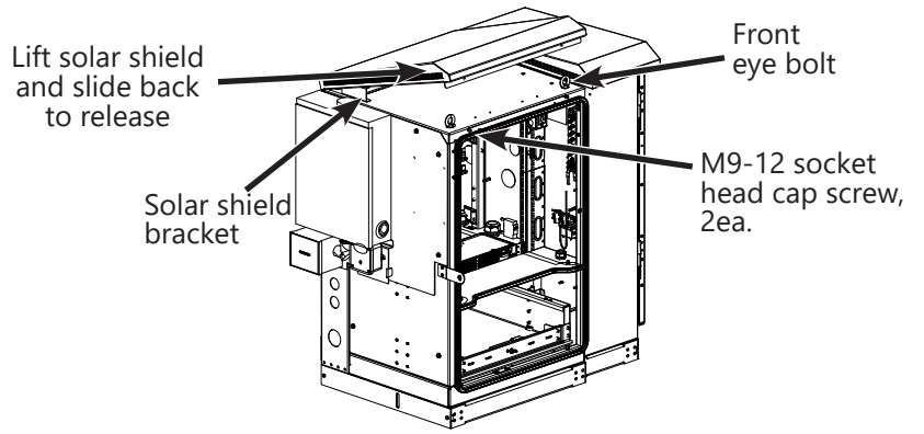
Figure 17. Solar Shield Removal
