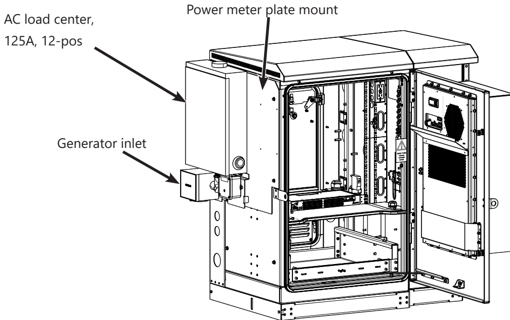
Figure 4. Left Side Views with 125Amp AC Load Center, CommScope Telco AIO Example
