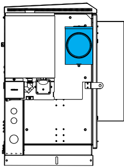
Figure 28. Structurally mounting power meters
