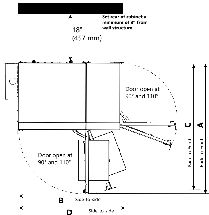
Figure 7. Top View, Door at 90° and 110° for CommScope Telco AIO
