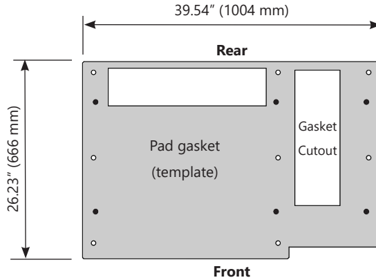
Figure 18. Gasket (Template) Required Between Cabinet and Pad or Vault
