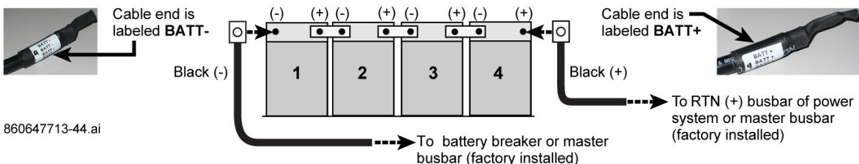
Figure 32. Battery String Cable Connections, Example with Lugs
