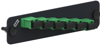
Adapter Pack, Black, 1000-Type, with 6 Singlemode duplex LC/APC Adapters, green, no shutter
