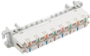
HighBand® Switching Module, with jumper rings, 16-pair, ivory
