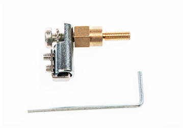
FIST® Universal cable termination kit, central strength member bracket, 12 pcs
