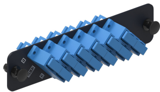
Adapter Pack, Black, 1000-Type, with 6 TeraSPEED® Singlemode duplex SC adapters, blue
