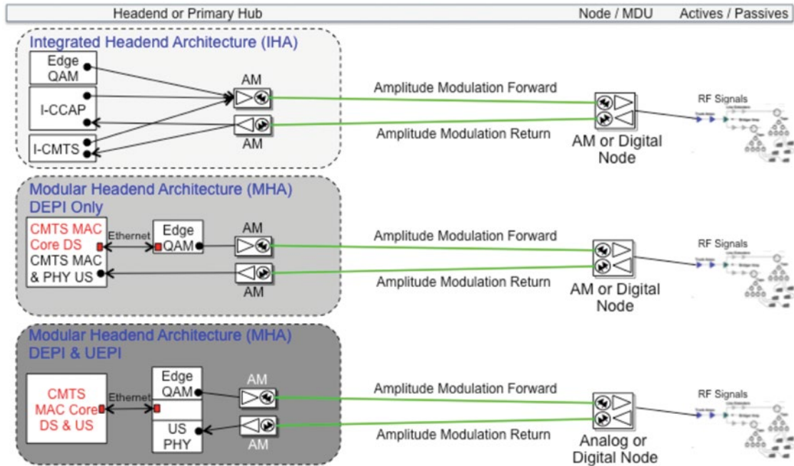
Figure 16: Summary Digital Video and DOCSIS MAC and PHY Functions for the Downstream
