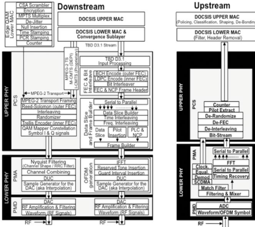
Figure 13: Functional Review of the RF MAC/PHY Layers Downstream and Upstream
