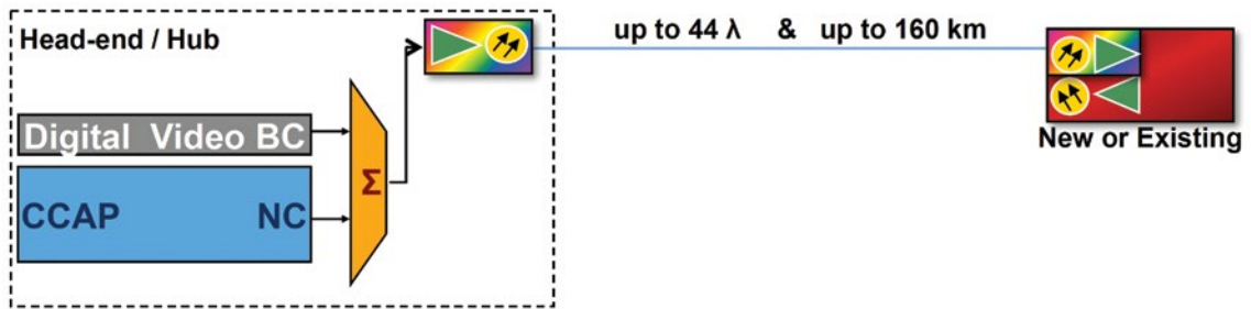
Figure 21: BCF Enables a Digital Transport for I-CCAP
