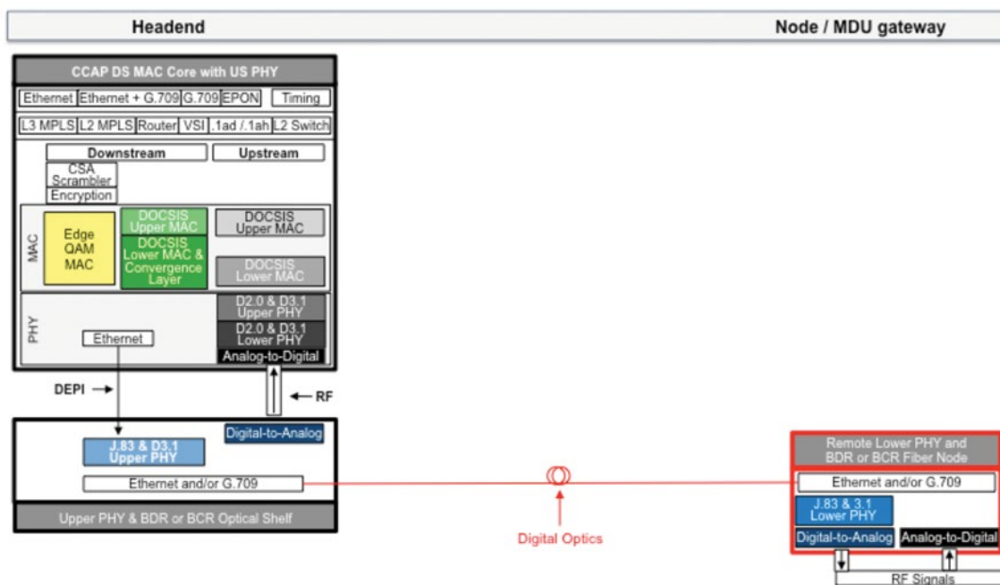
Figure 24: Remote Lower PHY and BDR Separate Headend Optical Shelf Architecture
