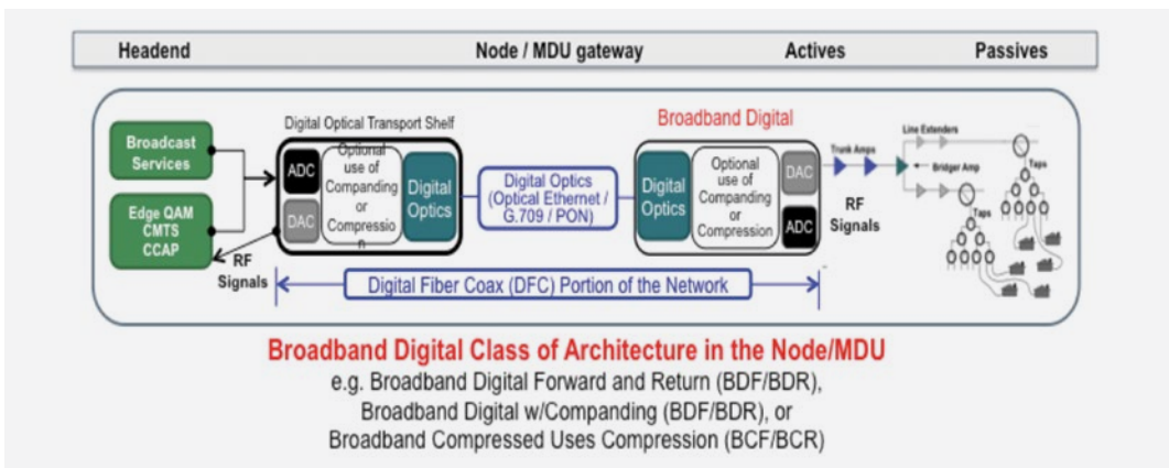
Figure 9: Digital Fiber Coax—Broadband Digital Class
