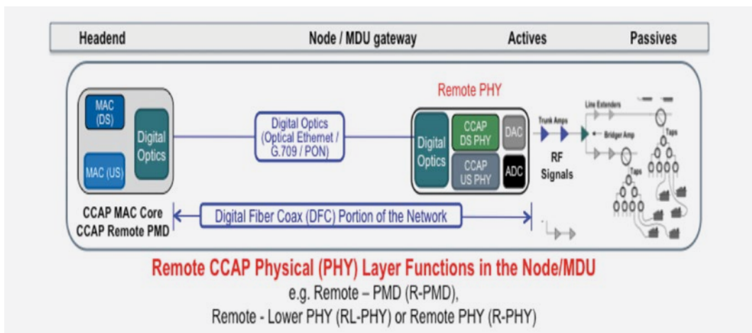
Figure 10: Digital Fiber Coax—Remote PHY CCAP Class
