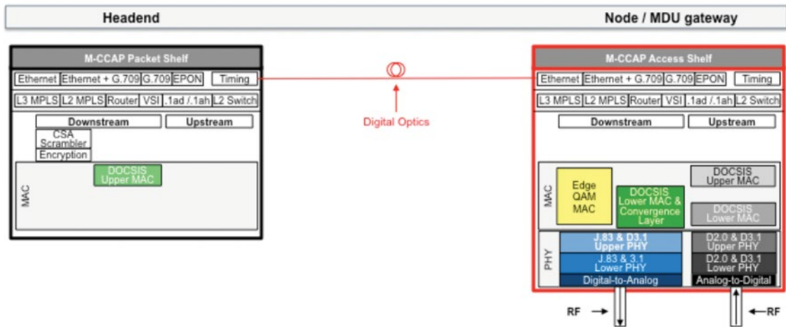
Figure 27: Remote Access Shelf (R-AS) Architecture
