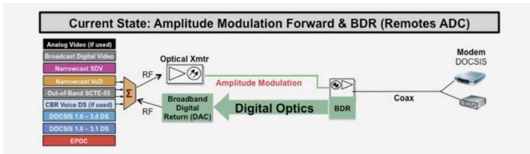
Figure 8: HFC Amplitude Modulation Forward and DFC Broadband Digital Return (BDR)
