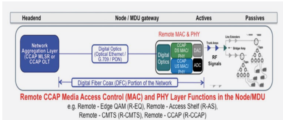
Figure 11: Digital Fiber Coax – Remote MAC and PHY Class
