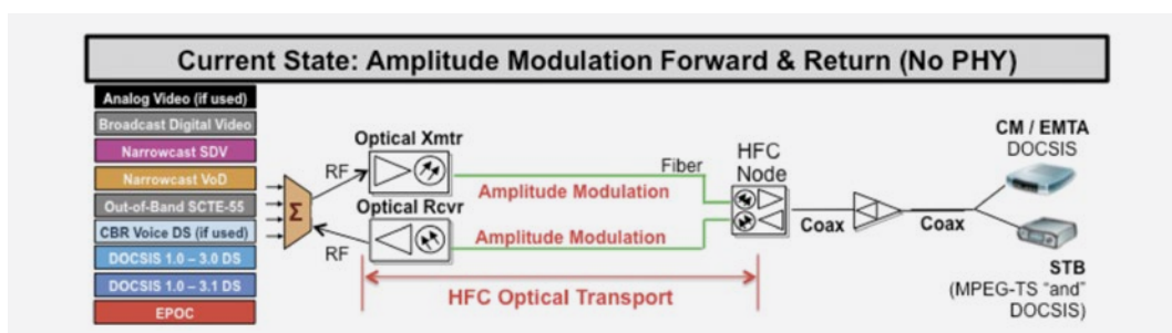
Figure 7: HFC Amplitude Modulation Forward and Return
