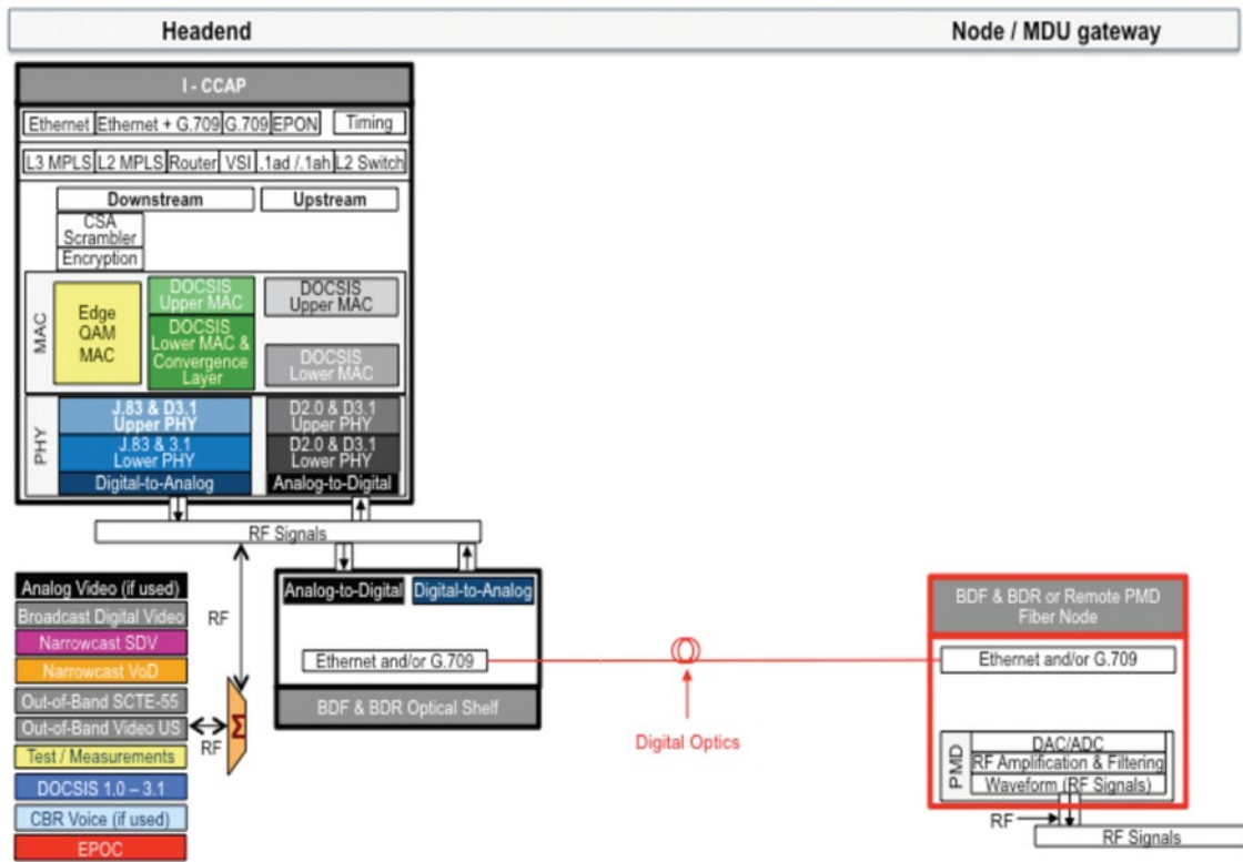
Figure 18: Broadband Digital Return and Forward Architecture
