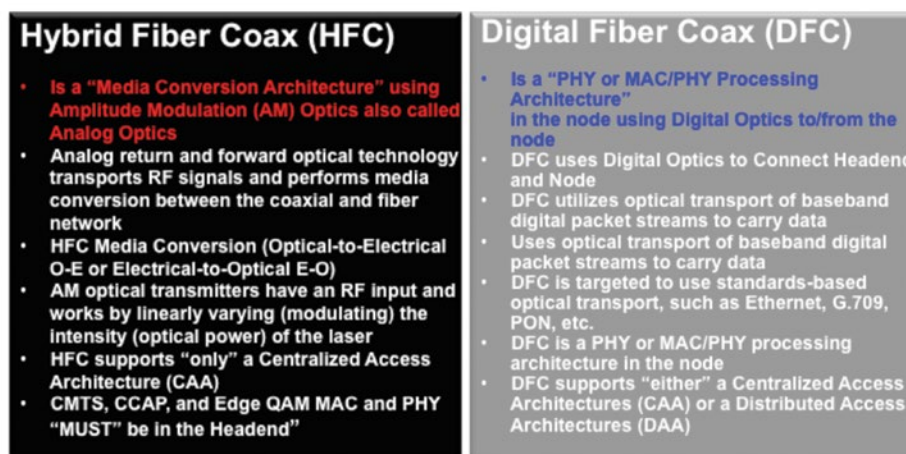
Figure 3: Descriptions of the Two Different FTTN Classes
