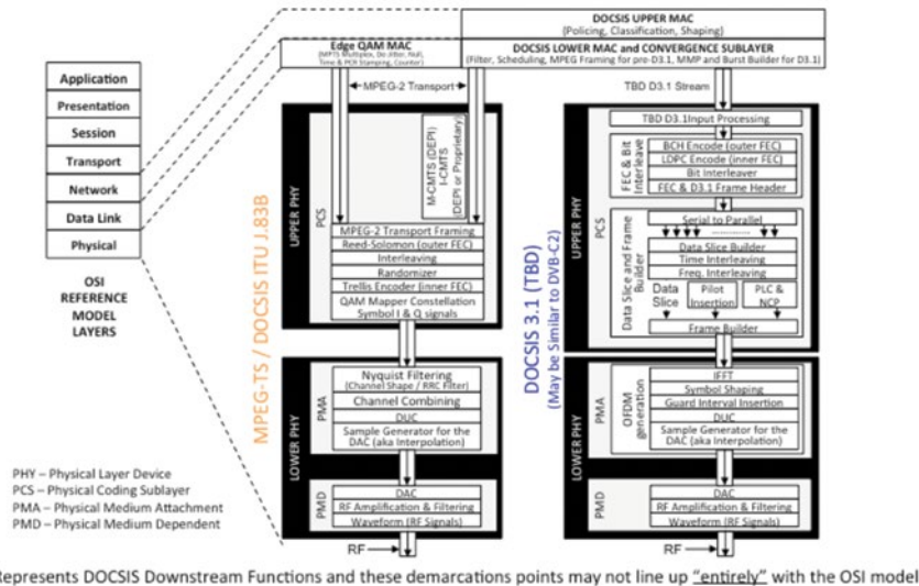
Figure 12: Detailed Digital Video and DOCSIS MAC and PHY Functions for the Downstream
