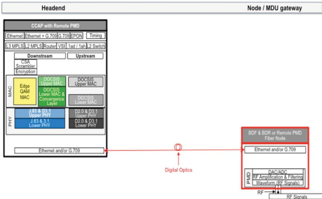
Figure 22: Remote PMD Architecture
