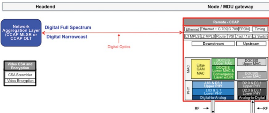
Figure 28: Remote CCAP (R-CCAP) Architecture
