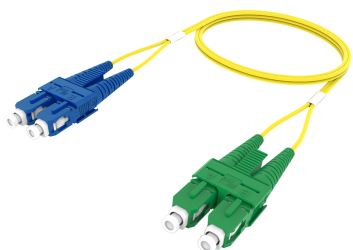
Fiber Optic Patch Cord, Duplex, Singlemode, SC/UPC to SC/APC, yellow, 10 m
