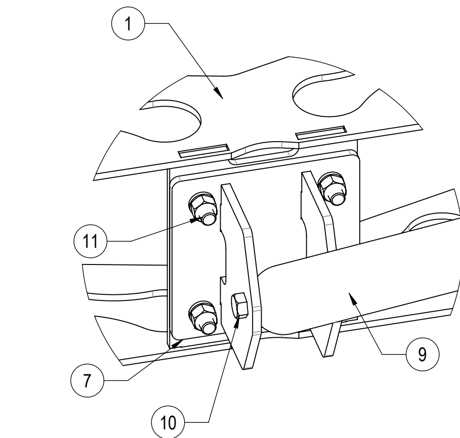
DETAIL B SCALE 1 : 4
