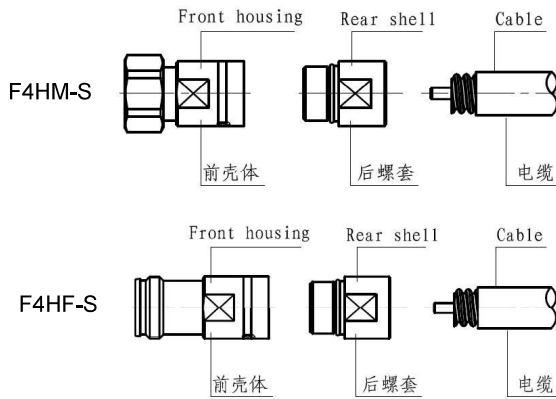
连接器及电缆配件图 Connector and cable accessories
